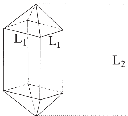
Figure 8. Characteristic lengths of KDP crystals.
