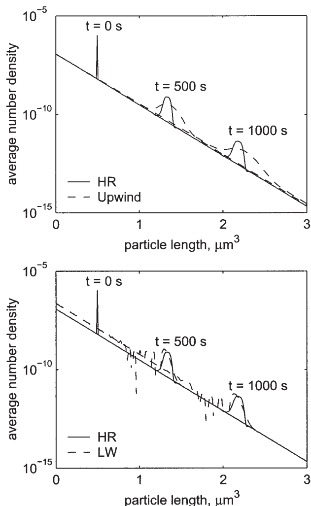
Figure 15. High-resolution, the upwind, and the Lax-Wendroff simulations for a spike perturbation (Example 5).
